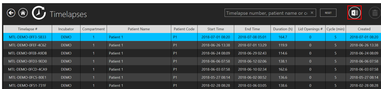
Figure 7.7 “Report” button
