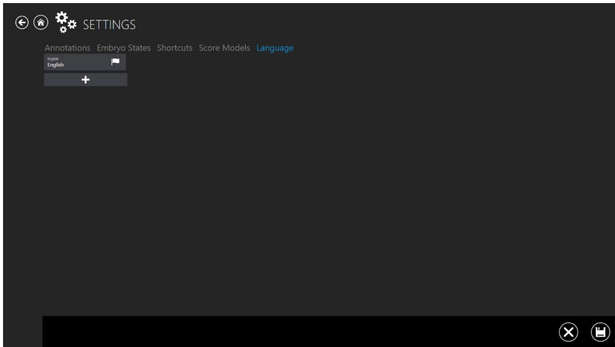
Figure 7.178 Language submenu
