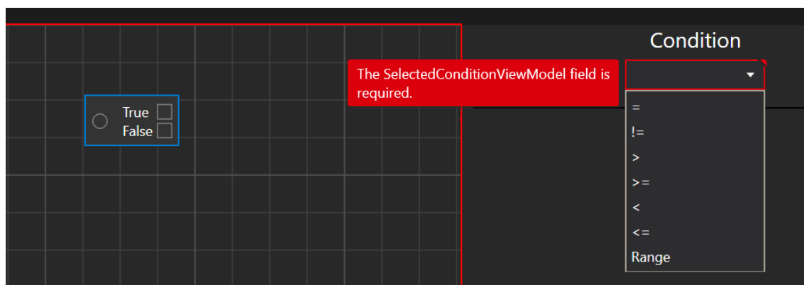
Figure 7.156 Available conditions
