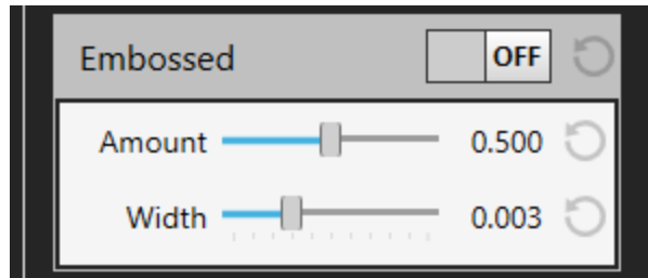
Figure 7.94 Embossed settings
