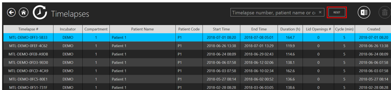
Figure 7.6 “Reset” button
