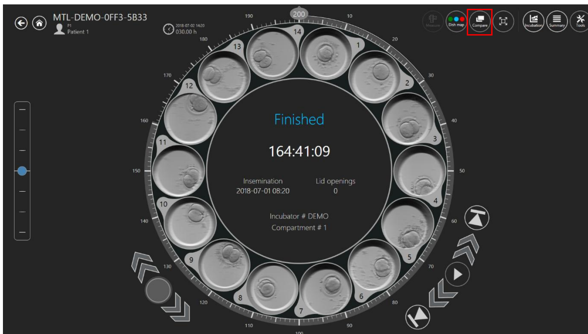
Figure 7.38 “Compare” button
