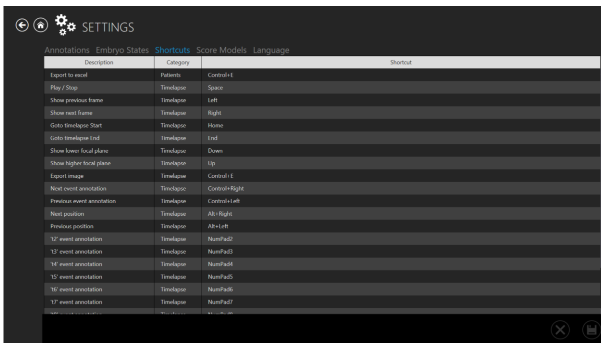
Figure 7.141 Shortcuts submenu
