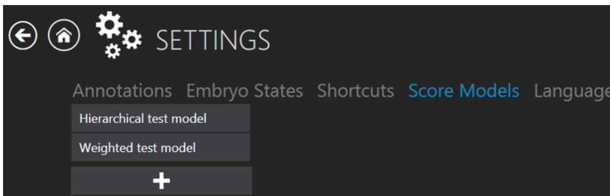
Figure 7.144 Score models
