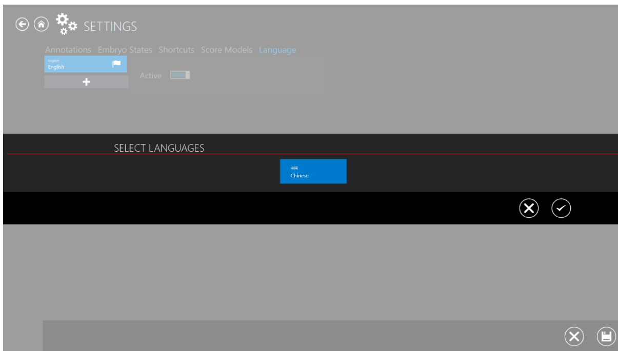
Figure 7.179 Language options
