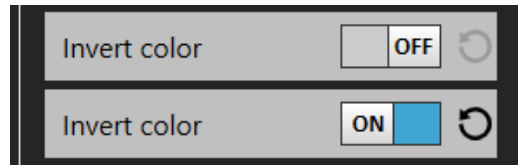
Figure 7.98 “ON/OFF” button
