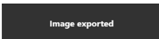
Figure 7.79 Exporting confirmation
