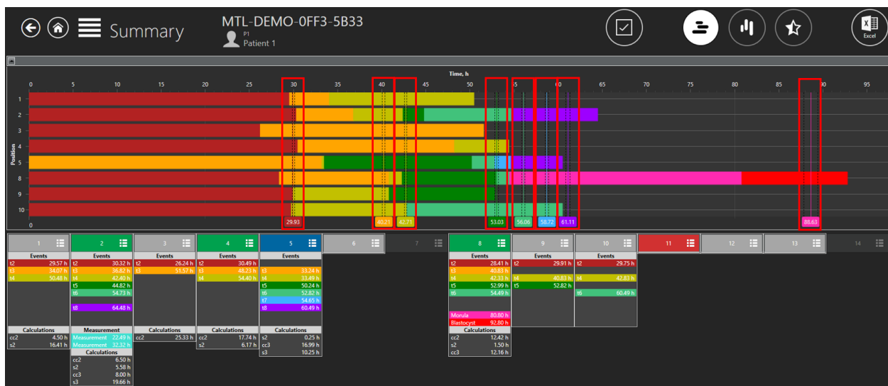
Figure 7.51 Ideal times
