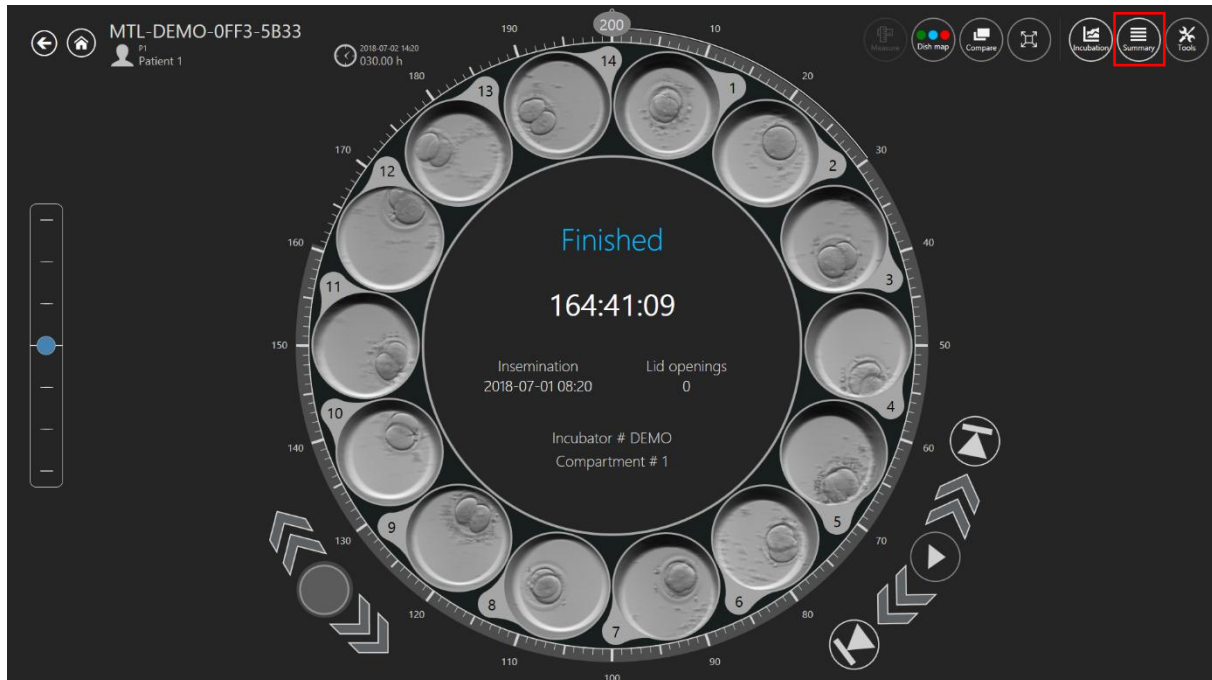
Figure 7.49 “Summary” button
