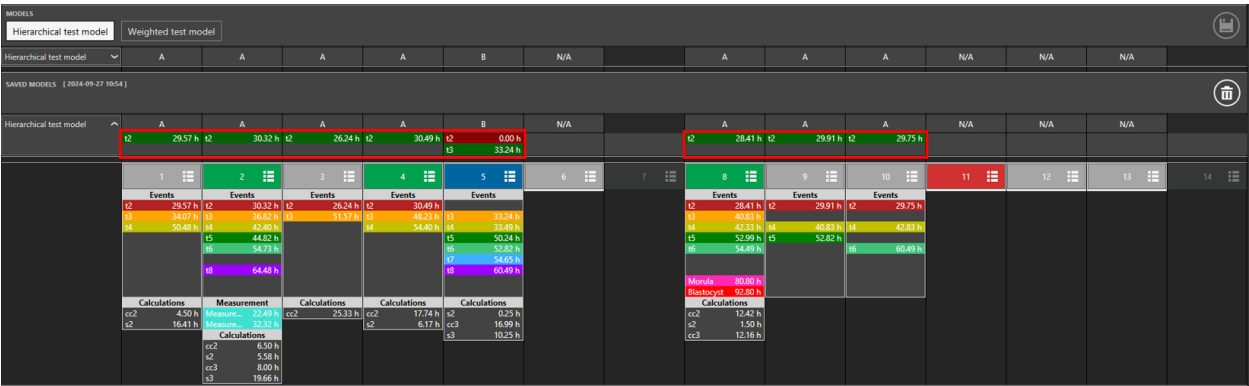
Figure 7.64 List of all conditional nodes that are created in the hierarchical score model
